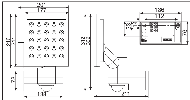
XLED 25
