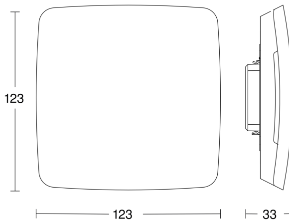
Dimension Drawing
