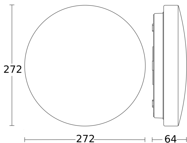
Dimension Drawing
