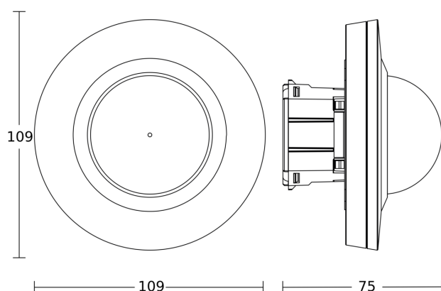
Dimension Drawing 1
