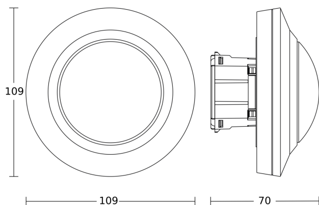
Dimension Drawing 1
