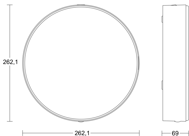
Dimension Drawing
