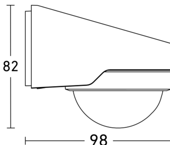
Dimension Drawing 2
