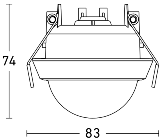
Dimension Drawing
