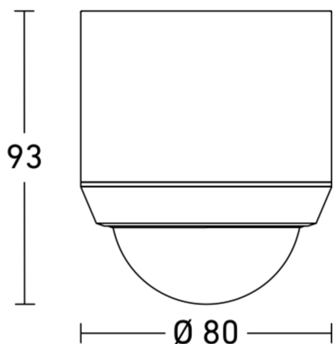
Dimension Drawing
