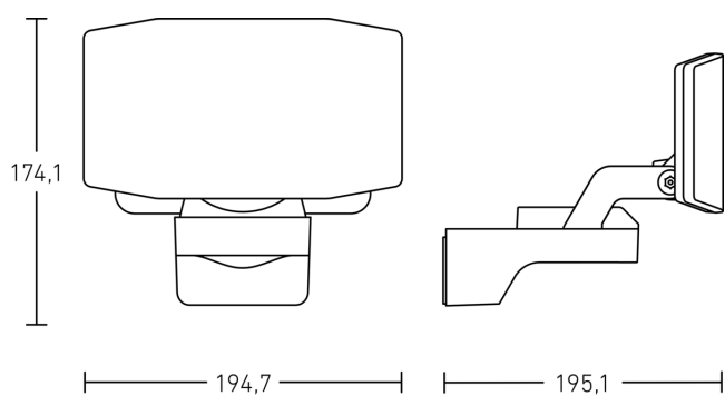
Dimension Drawing
