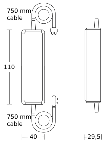
Dimension Drawing 2
