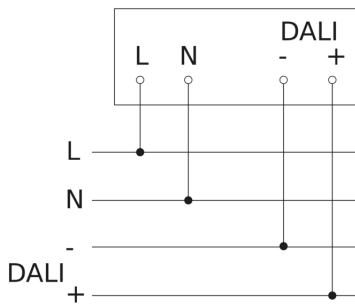
Master circuit diagram
