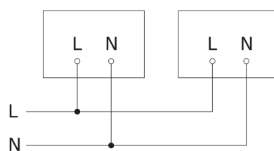
Master/master interconnection circuit diagram
