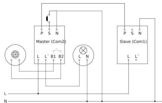
Master/slave interconnection circuit diagram
