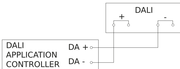
Circuit diagram
